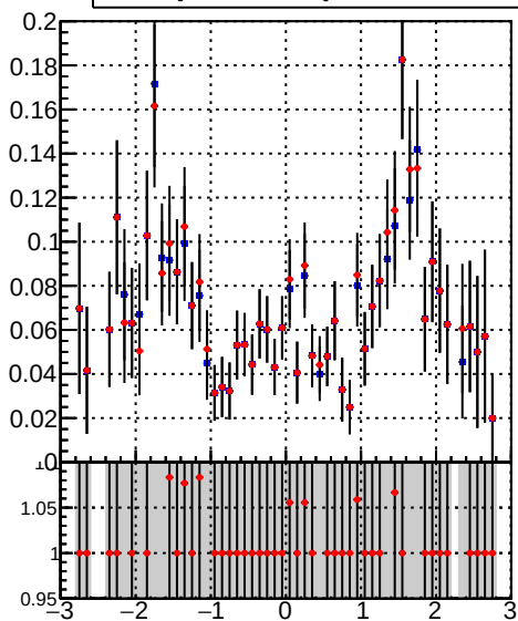
■ DQM_TT_mkFit-DQM_original ■ DQM_TT_mkFit-DQM_modified
