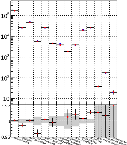
Number —●— DQM_TT_mkFit-DQM_modified
