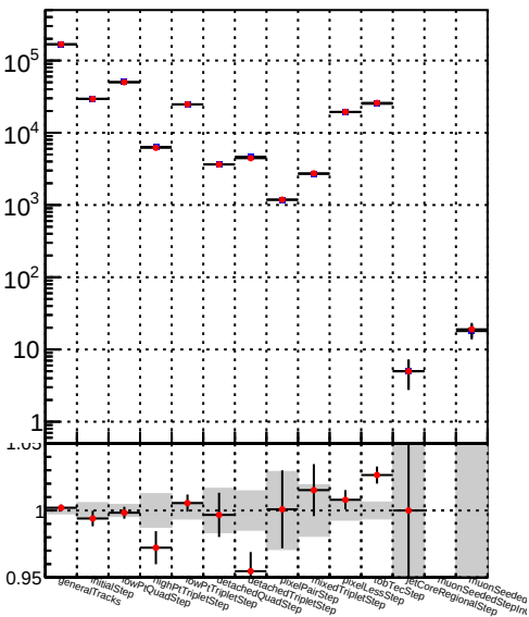
Number —●— DQM_TT__mkFit-DQM_modified
