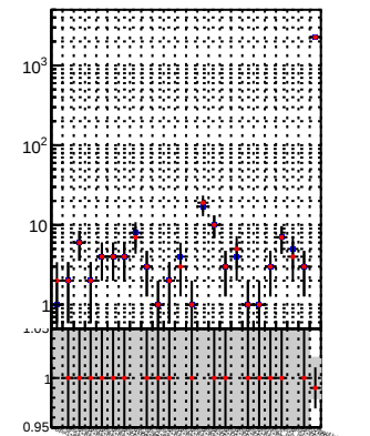
N of reco track vs. \chi^2
