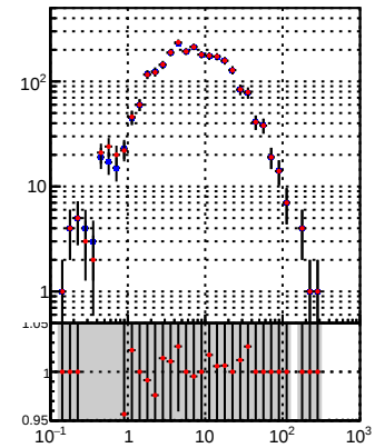
—●— DQM_TT_mkFit-DQM_original —●— DQM_TT_mkFit-DQM_modified
