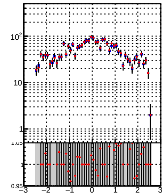
—●— DQM_TT_mkFit-DQM_original —●— DQM_TT_mkFit-DQM_modified
