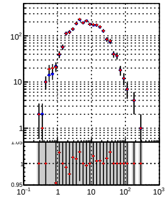
—●— DQM_TT_mkFit-DQM_original —●— DQM_TT_mkFit-DQM_modified
