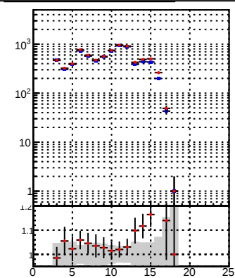
DQM_TT_mkFit-DQM_original DQM_TT_mkFit-DQM_modified
