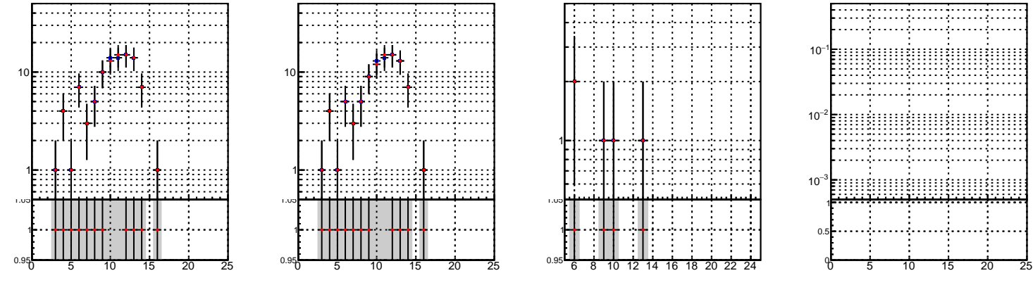
Legend: ■ DQM_TT_mkFit-DQM_original ■ DQM_TT_mkFit-DQM_modified
