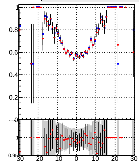
—■— DQM_TT_mkFit-DQM_original —●— DQM_TT_mkFit-DQM_modified
