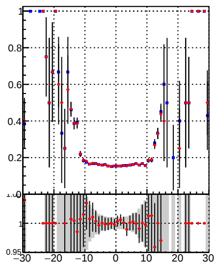
Fake rate vs d —●— DQM TT mkFit-DQM_original —●— DQM TT mkFit-DQM_modified
