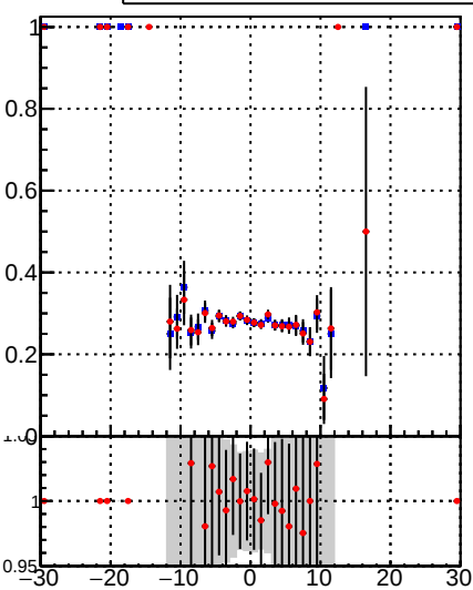
■ DQM_TT_mkFit-DQM_original ● DQM_TT_mkFit-DQM_modified
