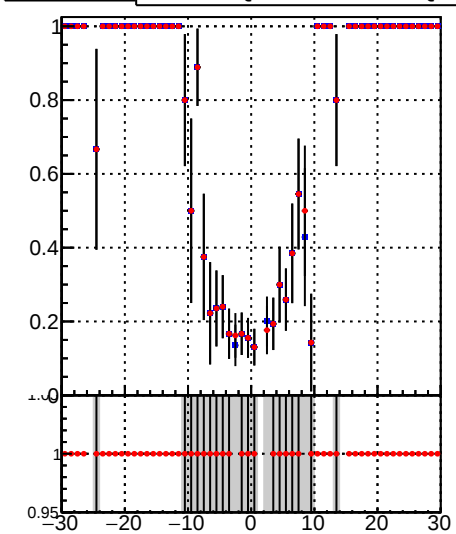
—•— DQM_TT_mkFit-DQM_original —•— DQM_TT_mkFit-DQM_modified
