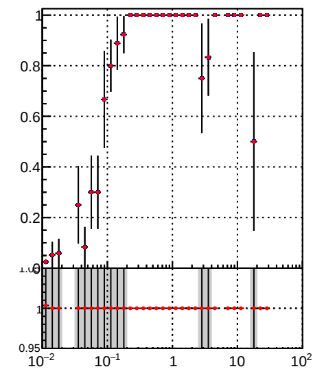
—•— DQM_TT_mkFit-DQM_original —•— DQM_TT_mkFit-DQM_modified
