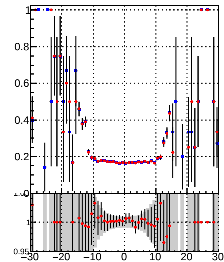
■ DQM_TT_mkFit-DQM_original ■ DQM_TT_mkFit-DQM_modified
