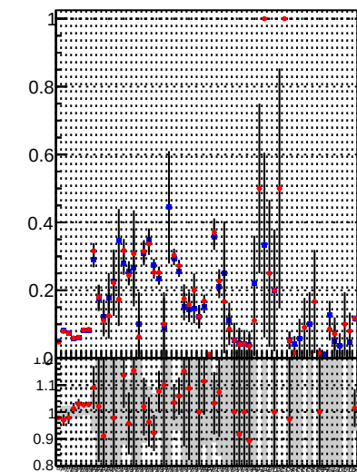
Fake rate vs. —●— DQM TT mkFit-DQM_original —●— DQM TT mkFit-DQM_modified
