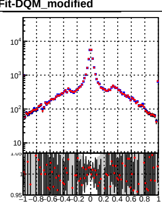
█ DQM_TT_mkFit-DQM_original █ DQM_TT_mkFit-DQM_modified
