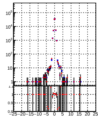
█ DQM_TT_mkFit-DQM_original █ DQM_TT_mkFit-DQM_modified
