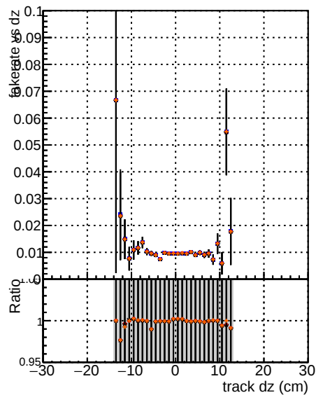
Fake rate vs d — BSM mktFit newBASE3 — BSM mktFit newNDP — BSM mktFit newORR
