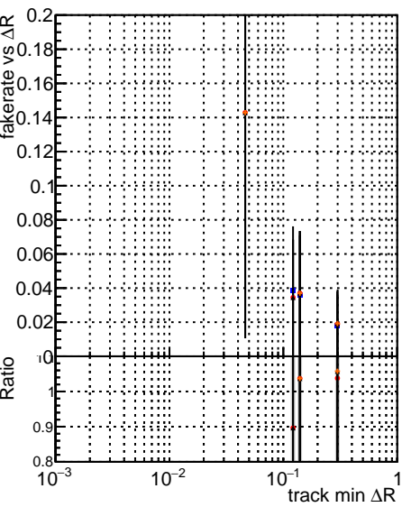
Fake rate vs \Delta R(\text{track, jet}) —●— DQM mkFit newBASE3 —●— DQM mkFit newANDPL —●— DQM mkFit newOKKK
