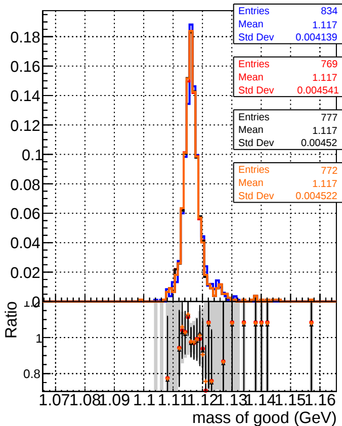
Mass of good Lambda
