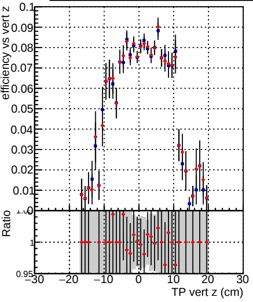
Efficiency vs TP vert z (cm) Legend: DQM_TT_mkFit-DQM_original-lowpt (blue diamonds) DQM_TT_mkFit-DQM_updated-lowpt (red circles)
