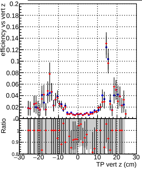
Efficiency vs vert z Legend: DQM_TT_mkFit-DQM_original-lowpt (blue squares) DQM_TT_mkFit-DQM_updated-lowpt (red circles)
