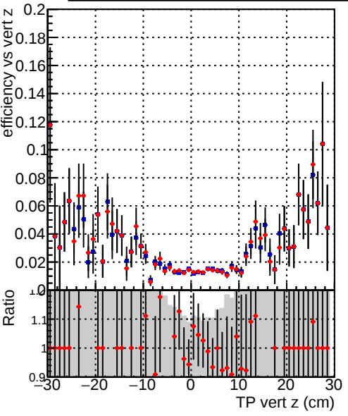
Efficiency vs vert z Legend: DQM_TT_mkFit-DQM_original-lowpt DQM_TT_mkFit-DQM_updated-lowpt
