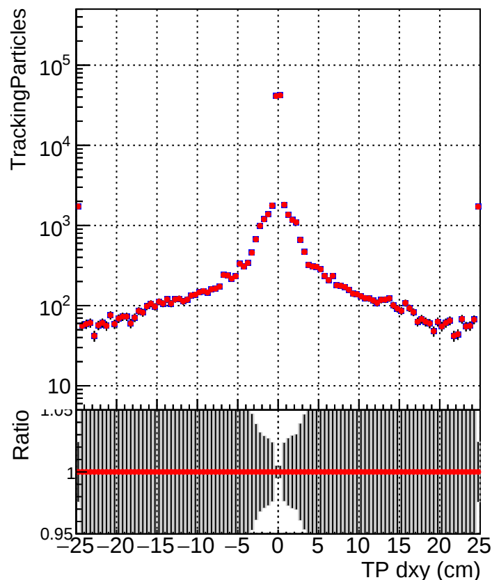
DQM_TT_mkFit-DQM_original-lowpt DQM_TT_mkFit-DQM_updated-lowpt
