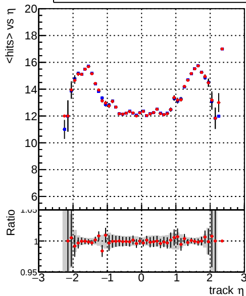
mean hits vs \eta Legend: DQM_TT_mkFit-DQM_original-lowpt (blue line), DQM_TT_mkFit-DQM_updated-lowpt (red line)
