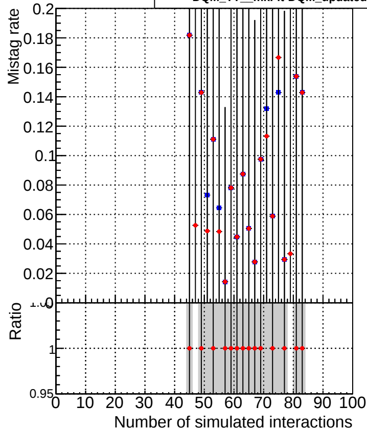
—•— DQM_TT_mkFit-DQM_original-lowpt —•— DQM_TT_mkFit-DQM_updated-lowpt
