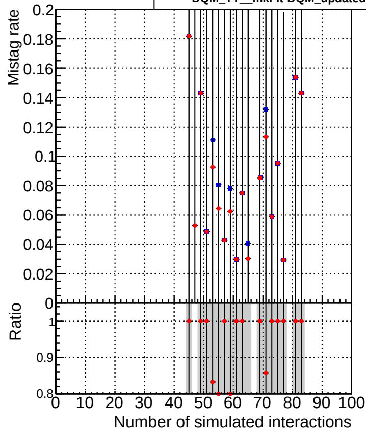
■ DQM_TT_mkFit-DQM_original-lowpt ● DQM_TT_mkFit-DQM_updated-lowpt
