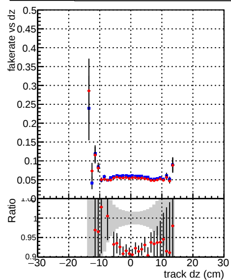
Fake rate vs dz —•— DQM TT mkFit-DQM_original-lowpt —•— DQM TT mkFit-DQM_updated-lowpt
