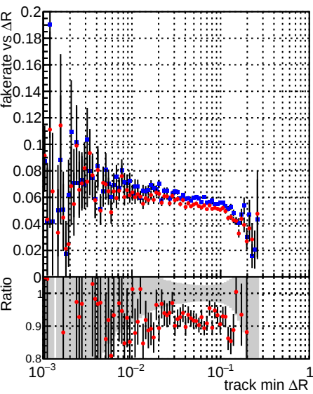
Legend: DQM_TT_mkFit-DQM_original-lowpt (blue squares), DQM_TT_mkFit-DQM_updated-lowpt (red circles)
