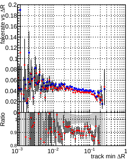
Fake rate vs \Delta R(\text{track}, \text{jet}) Legend: DQM_TT_mkFit-DQM_original-lowpt (blue) DQM_TT_mkFit-DQM_updated-lowpt (red)
