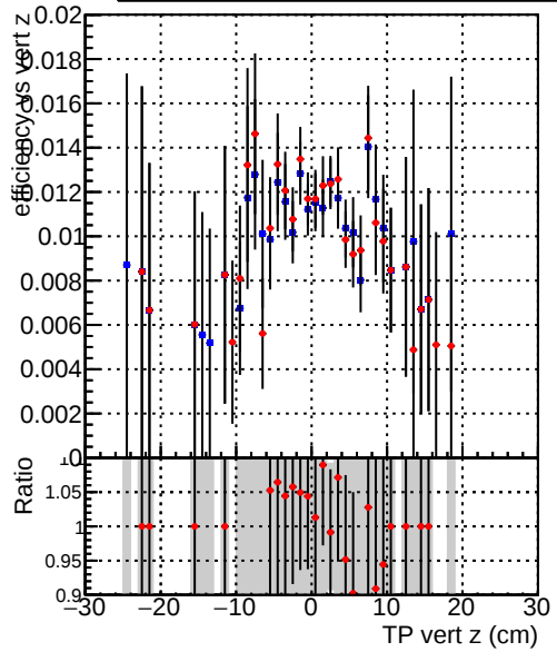
Efficiency vs vert z — DQM_TT_mkFit-DQM_original-lowpt — DQM_TT_mkFit-DQM_updated-lowpt
