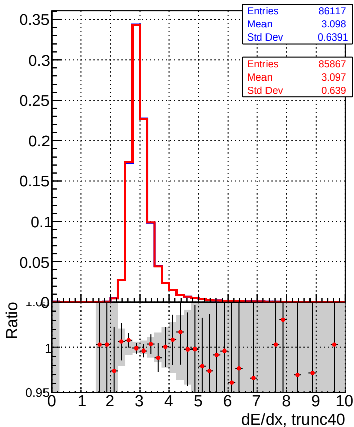
■ DQM_TT_mkFit-DQM_original-lowpt ● DQM_TT_mkFit-DQM_updated-lowpt
