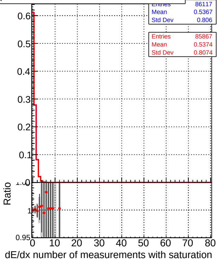
■ DQM_TT_mkFit-DQM_original-lowpt ● DQM_TT_mkFit-DQM_updated-lowpt
