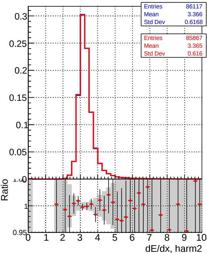
■ DQM_TT_mkFit-DQM_original-lowpt ● DQM_TT_mkFit-DQM_updated-lowpt
