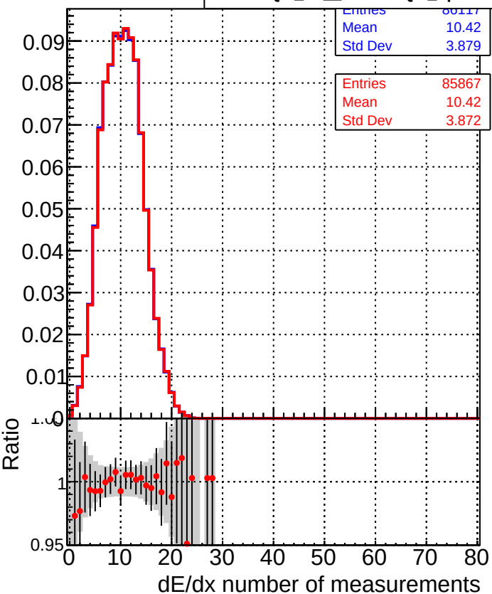
■ DQM_TT_mkFit-DQM_original-lowpt ● DQM_TT_mkFit-DQM_updated-lowpt
