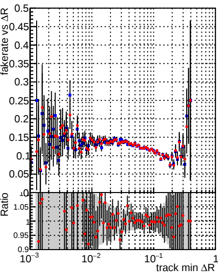
Legend: DQM_TT_mkFit-DQM_original-lowpt (blue), DQM_TT_mkFit-DQM_updated-lowpt (red)
