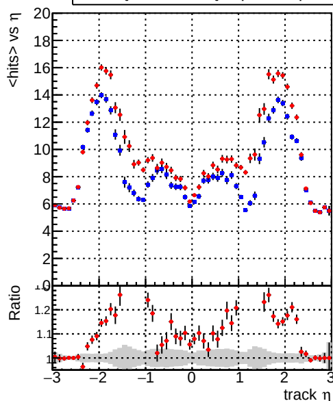
— DQM_TT_mkFit-DQM_original-lowpt — DQM_TT_mkFit-DQM_updated-lowpt
