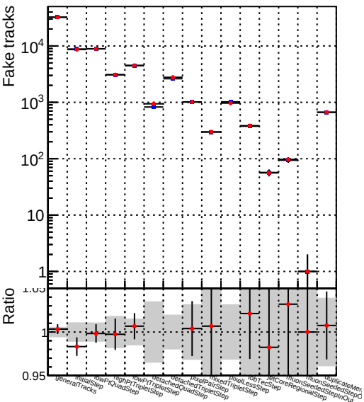
Number —●— DQM_TT_mkFit-DQM_updated-lowpt
