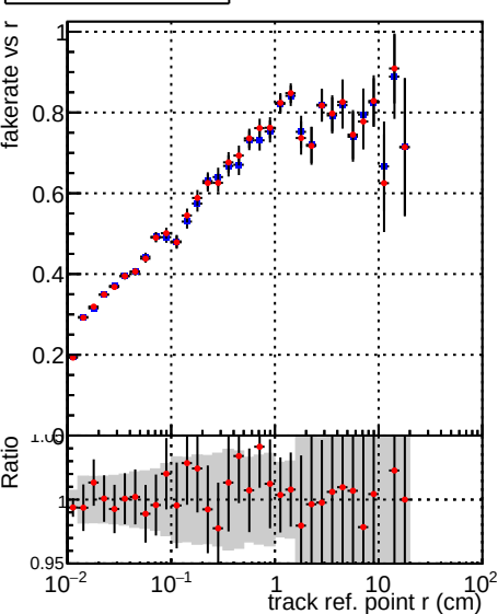
Fake rate vs vertpos Duplicates Rate vs vertpos Pileup rate vs vertpos
