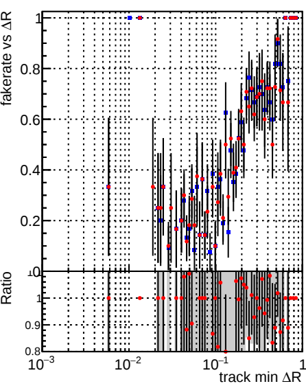
Fake rate vs \Delta R(\text{track, jet}) Legend: DQM_TT_mkFit-DQM_original-lowpt (blue squares) DQM_TT_mkFit-DQM_updated-lowpt (red circles)
