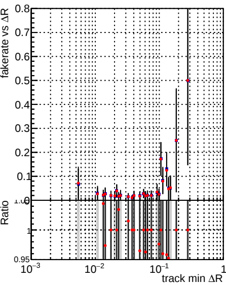
Fake rate vs \Delta R(\text{track, jet}) Legend: DQM_TT_mkFit-DQM_original-lowpt (grey line with blue dots) DQM_TT_mkFit-DQM_updated-lowpt (red line with red dots)
