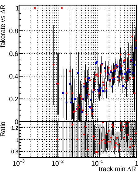
Fake rate vs \Delta R(\text{track, jet}) Legend: ■ DQM_TT_mkFit-DQM_original-lowpt ● DQM_TT_mkFit-DQM_updated-lowpt
