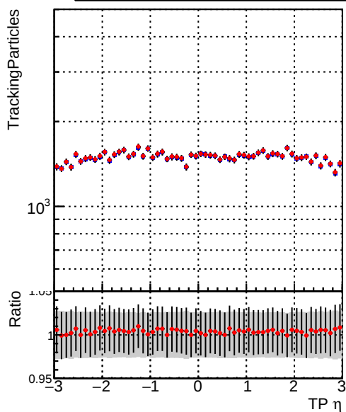
N of simulated tracks vs TP \eta —•— DQM_TT_mkFit-DQM_original-lowpt —•— DQM_TT_mkFit-DQM_updated-lowpt
