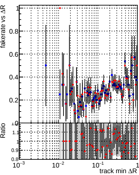
Fake rate vs \Delta R (track, jet) DQM_TT_mkFit-DQM_original-lowpt DQM_TT_mkFit-DQM_updated-lowpt
