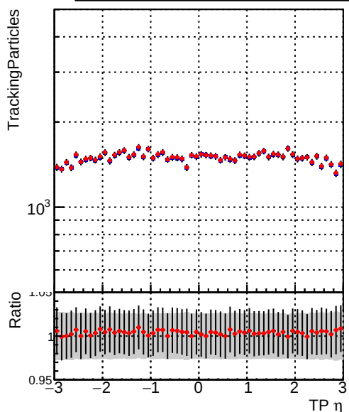
—•— DQM_TT_mkFit-DQM_original-lowpt —•— DQM_TT_mkFit-DQM_updated-lowpt
