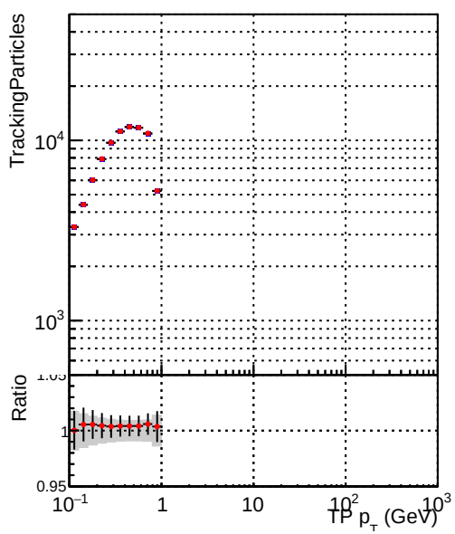
—•— DQM_TT_mkFit-DQM_original-lowpt —•— DQM_TT_mkFit-DQM_updated-lowpt
