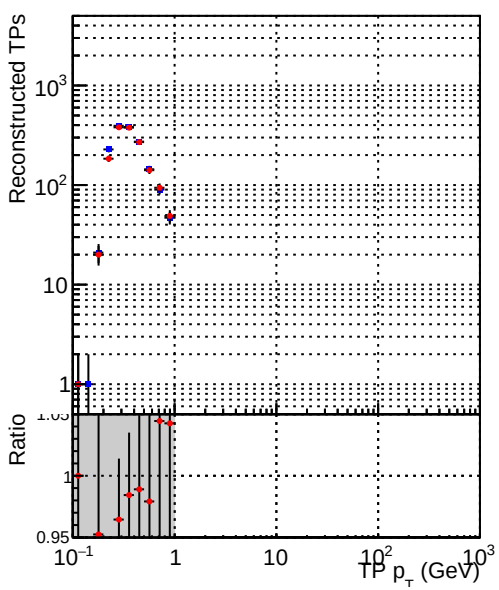
—•— DQM_TT_mkFit-DQM_original-lowpt —•— DQM_TT_mkFit-DQM_updated-lowpt
