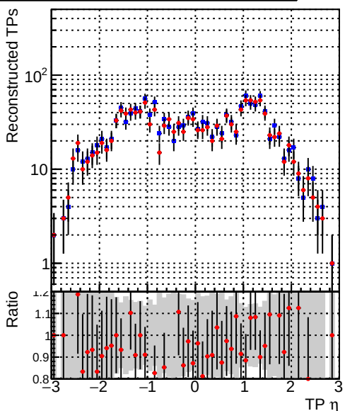
—•— DQM_TT_mkFit-DQM_original-lowpt —•— DQM_TT_mkFit-DQM_updated-lowpt
