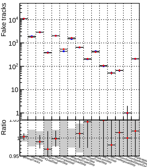
Number —●— DQM_TT__mkFit-DQM_updated-lowpt
