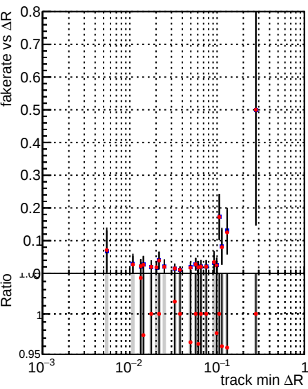
Fake rate vs ΔR(track, jet) DQM_TT_mkFit-DQM_original-lowpt DQM_TT_mkFit-DQM_updated-lowpt
