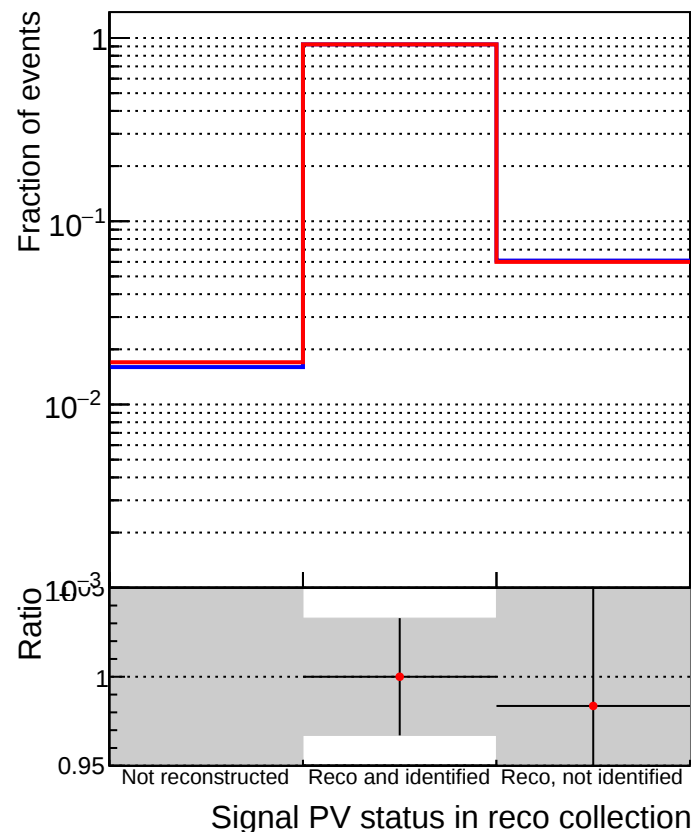
■ DQM_TT_mkFit-DQM_original-lowpt ● DQM_TT_mkFit-DQM_updated-lowpt
