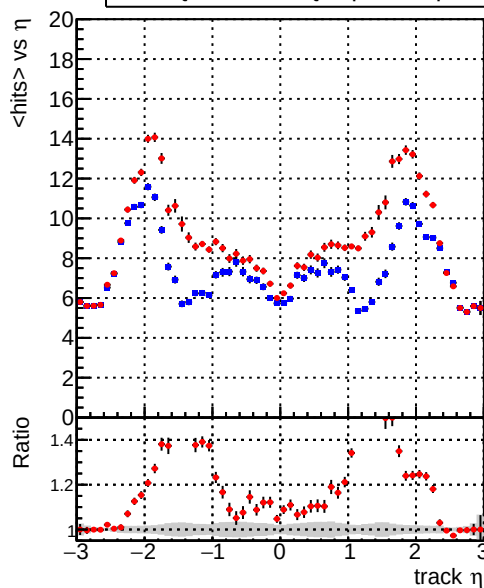
— DQM_TT_mkFit-DQM_original-lowpt — DQM_TT_mkFit-DQM_updated-lowpt
