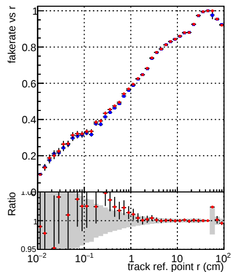
—•— DQM_TT_mkFit-DQM_original-lowpt —•— DQM_TT_mkFit-DQM_updated-lowpt
