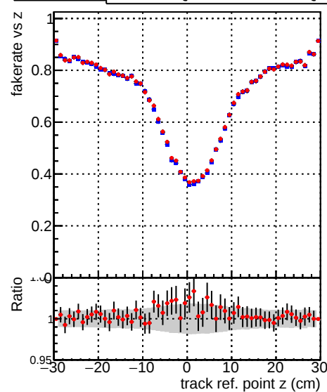
—•— DQM_TT_mkFit-DQM_original-lowpt —•— DQM_TT_mkFit-DQM_updated-lowpt
