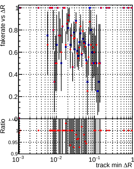
Fake rate vs \Delta R(\text{track, jet}) Legend: \blacksquare DQM_TT_mkFit-DQM_original-lowpt \bullet DQM_TT_mkFit-DQM_updated-lowpt
