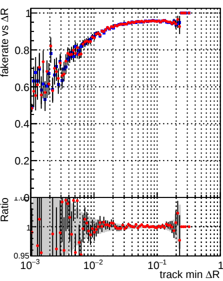
Fake rate vs \Delta R(\text{track, jet}) Legend: DQM_TT_mkFit-DQM_original-lowpt (blue circles) DQM_TT_mkFit-DQM_updated-lowpt (red circles)
