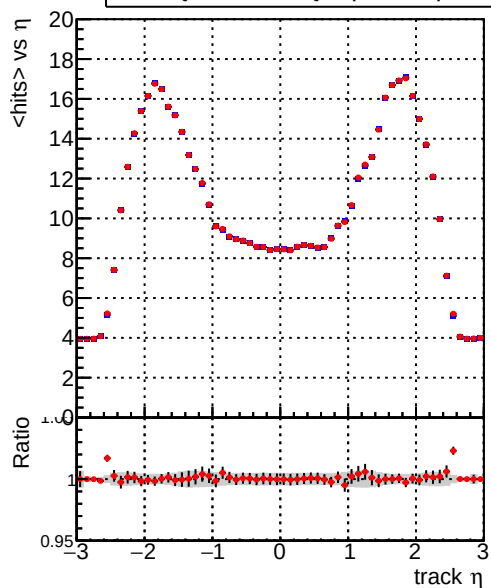
— DQM_TT_mkFit-DQM_original-lowpt — DQM_TT_mkFit-DQM_updated-lowpt
