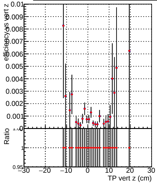
Efficiency vs. TP vert z (cm) — DQM_TT_mkFit-DQM_original-lowpt — DQM_TT_mkFit-DQM_updated-lowpt
