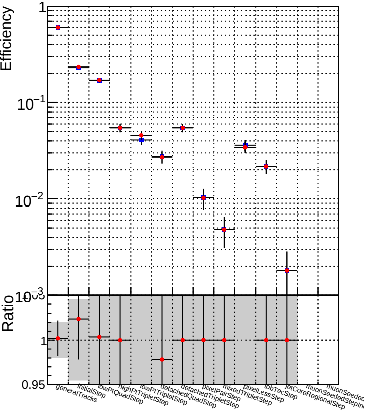
DQM_TT_mkFit-DQM_original-lowpt DQM_TT_mkFit-DQM_updated-lowpt
