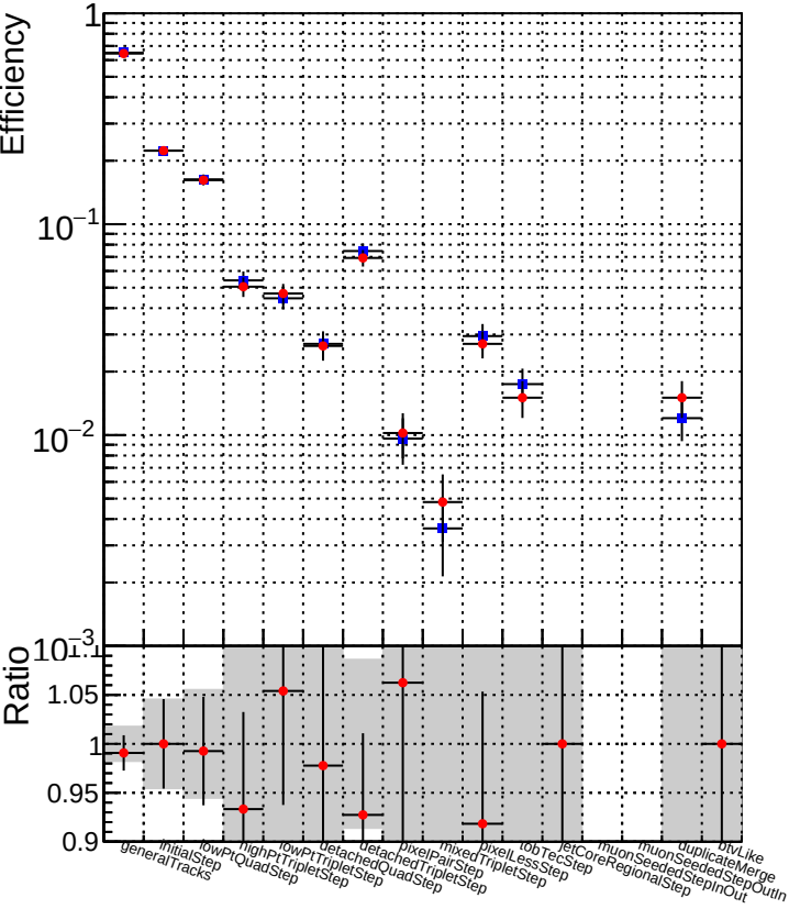
DQM_TT_mkFit-DQM_original-lowpt DQM_TT_mkFit-DQM_updated-lowpt
